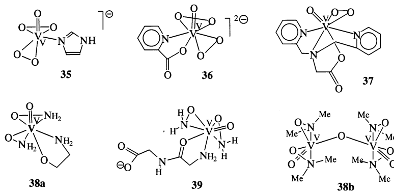
Fig. 13. Peroxo and hydroxylamido complexes of vanadium. 35 [60], 36 [61], 37 [51], 38a [62], 38b [64], 39 [62,63].
