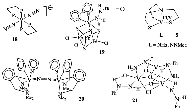
Fig. 7. Nitrogen activation and intermediates in \text{N}_2 fixation. 18 [33], 19 [35], 5 [20], 20 [36,37], 21 [38].
